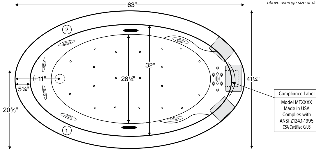
Numbered areas on tub deck represent possible locations to install cleaning systems, faucets and other fixtures.
