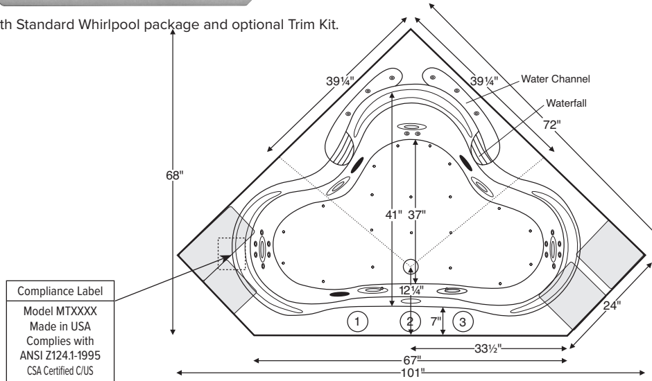
Numbered areas on tub deck represent possible locations to install cleaning systems, faucets and other fixtures.
