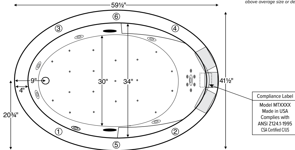
Numbered areas on tub deck represent possible locations to install cleaning systems, faucets and other fixtures.
