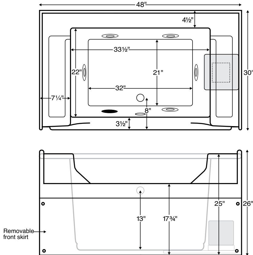
Pump and fixtures come standard on the right. Left-hand placement is available by special request.
