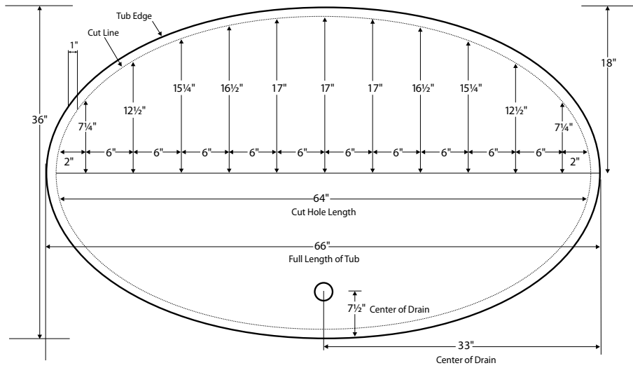
#123 Template Diagram
