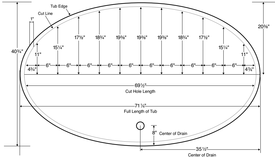
#117 Template Diagram
