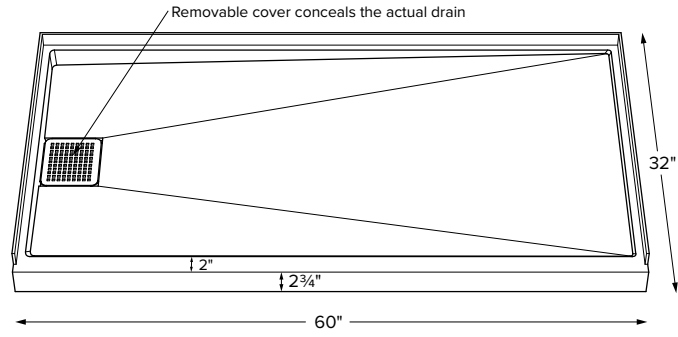
When ordering, please specify left- or right-hand drain and tile flange locations.
